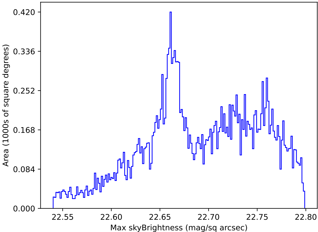
too_ignore_10_4v3.4_10yrs All sky u band: Max skyBrightness
