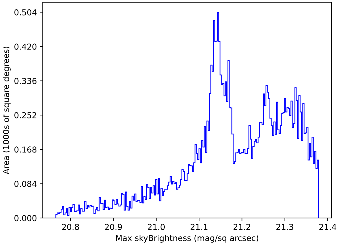
too_ignore_10_4v3.4_10yrs All sky r band: Max skyBrightness
