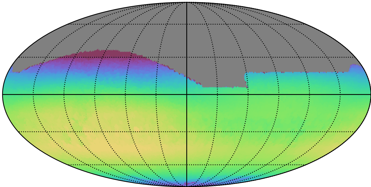
too_ignore_10_4v3.4_10yrs All sky i band: Max skyBrightness
