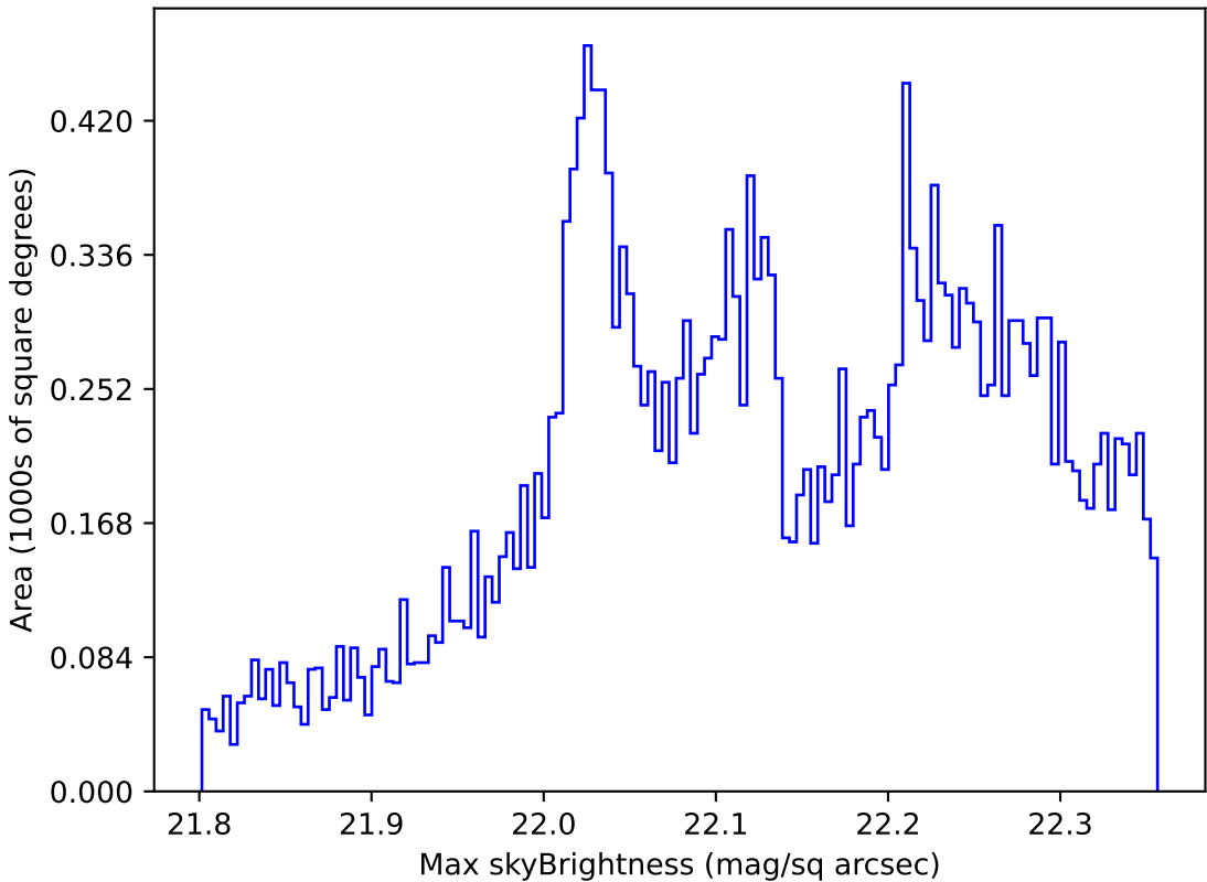
too_ignore_10_4v3.4_10yrs All sky g band: Max skyBrightness
