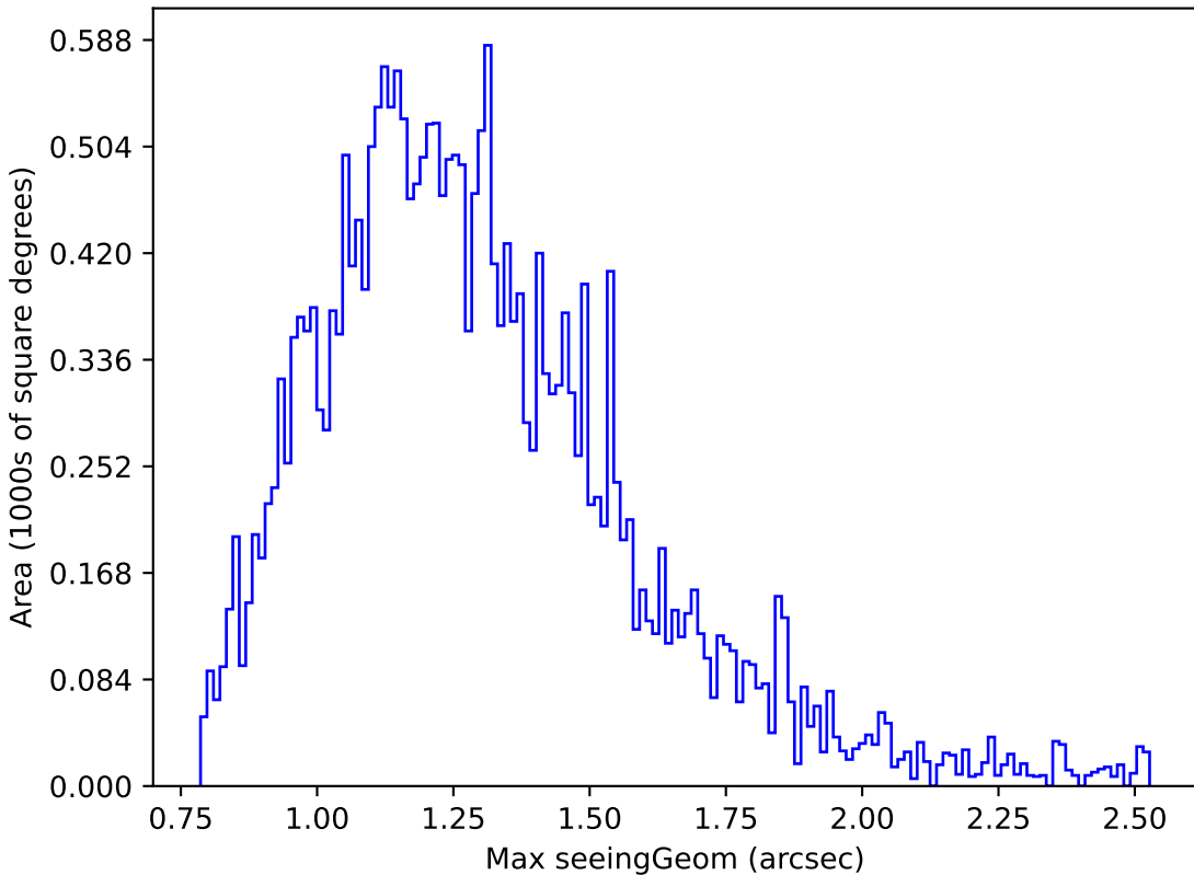
too_ignore_10_4v3.4_10yrs Yr 1 z band: Max seeingGeom
