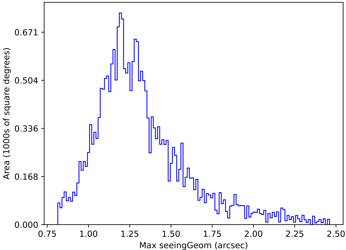
too_ignore_10_4v3.4_10yrs Yr 1 y band: Max seeingGeom
