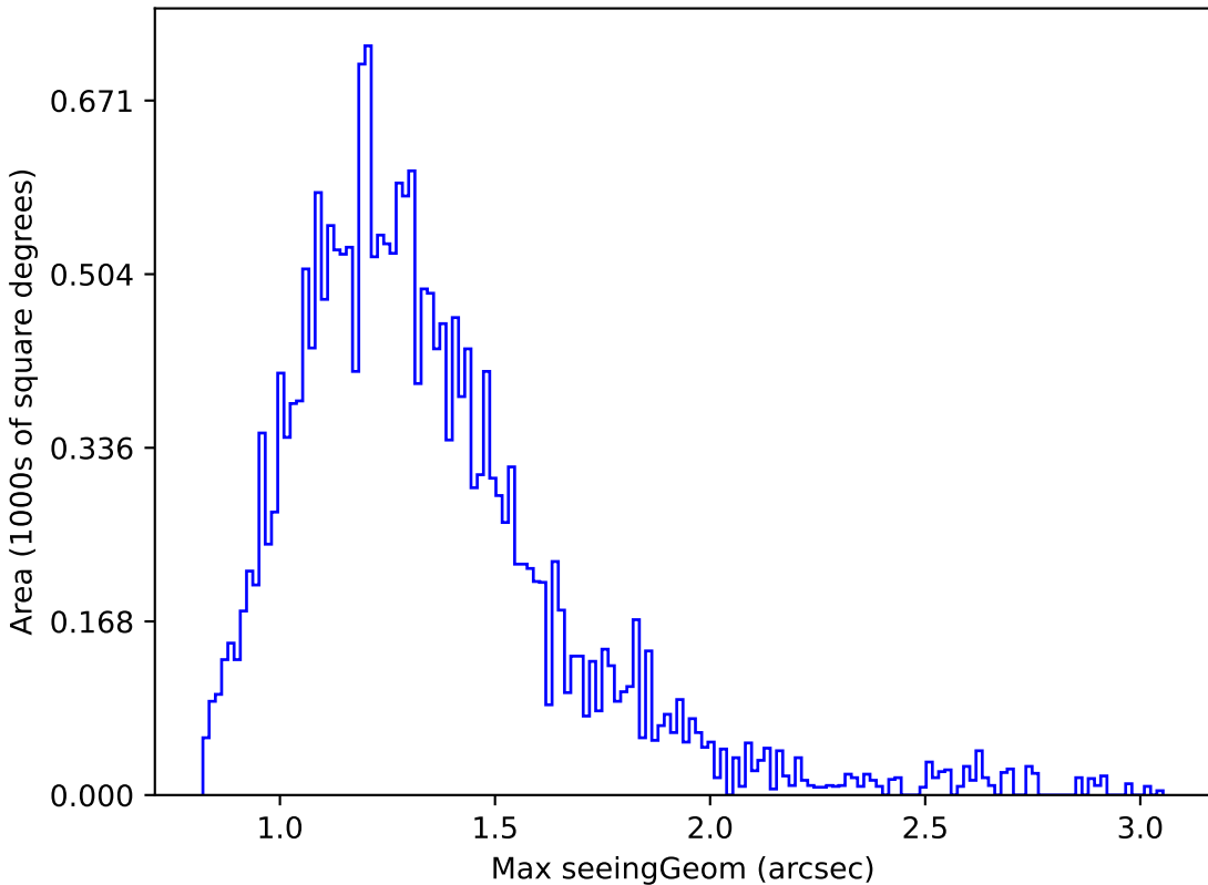
too_ignore_10_4v3.4_10yrs Yr 1 u band: Max seeingGeom
