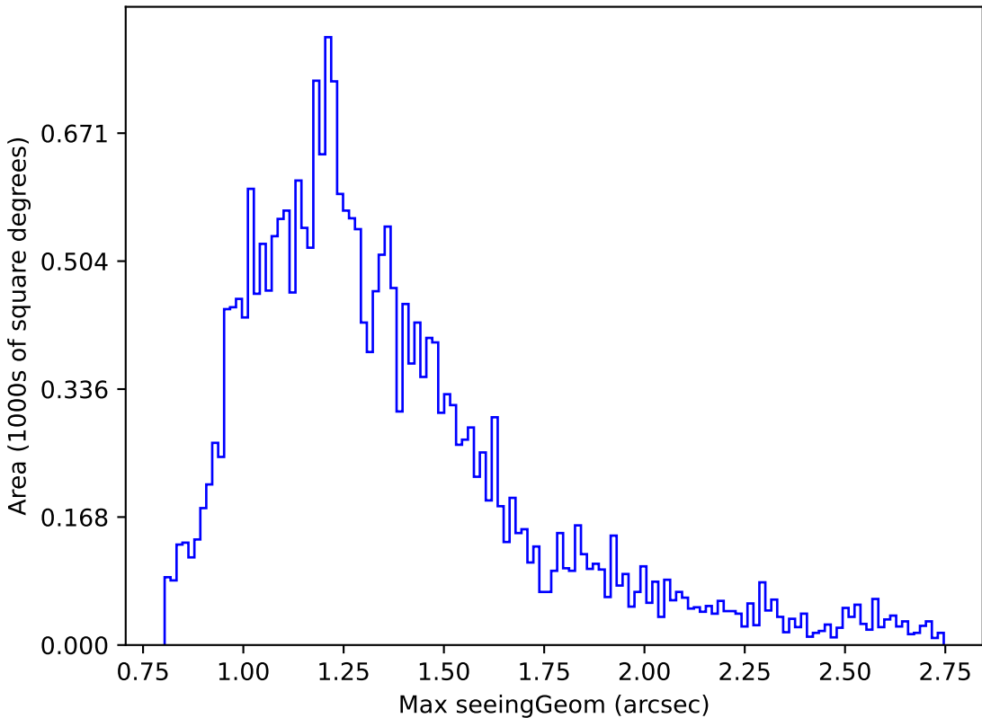
too_ignore_10_4v3.4_10yrs Yr 1 i band: Max seeingGeom
