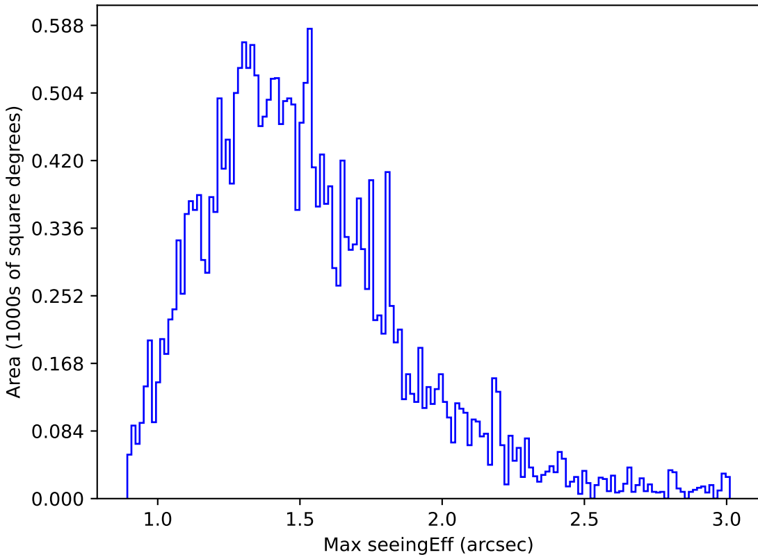
too_ignore_10_4v3.4_10yrs Yr 1 z band: Max seeingEff
