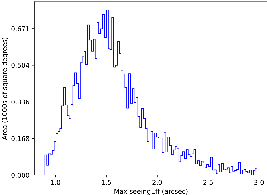
too_ignore_10_4v3.4_10yrs Yr 1 r band: Max seeingEff
