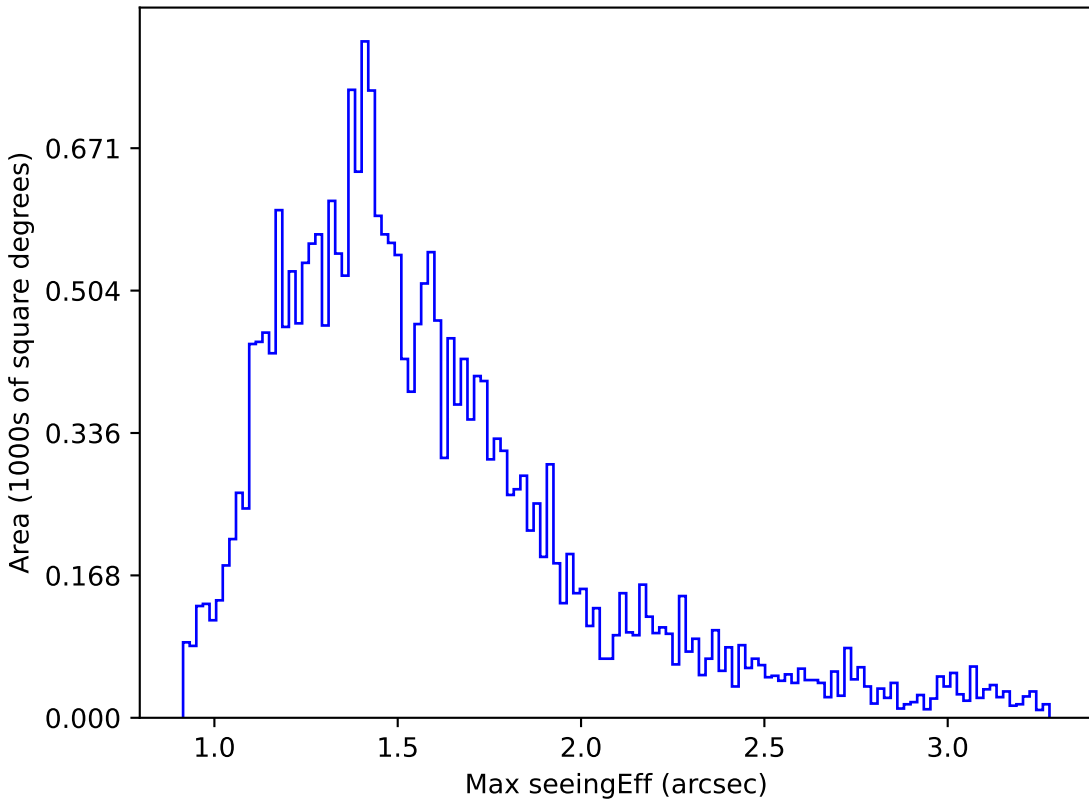
too_ignore_10_4v3.4_10yrs Yr 1 i band: Max seeingEff
