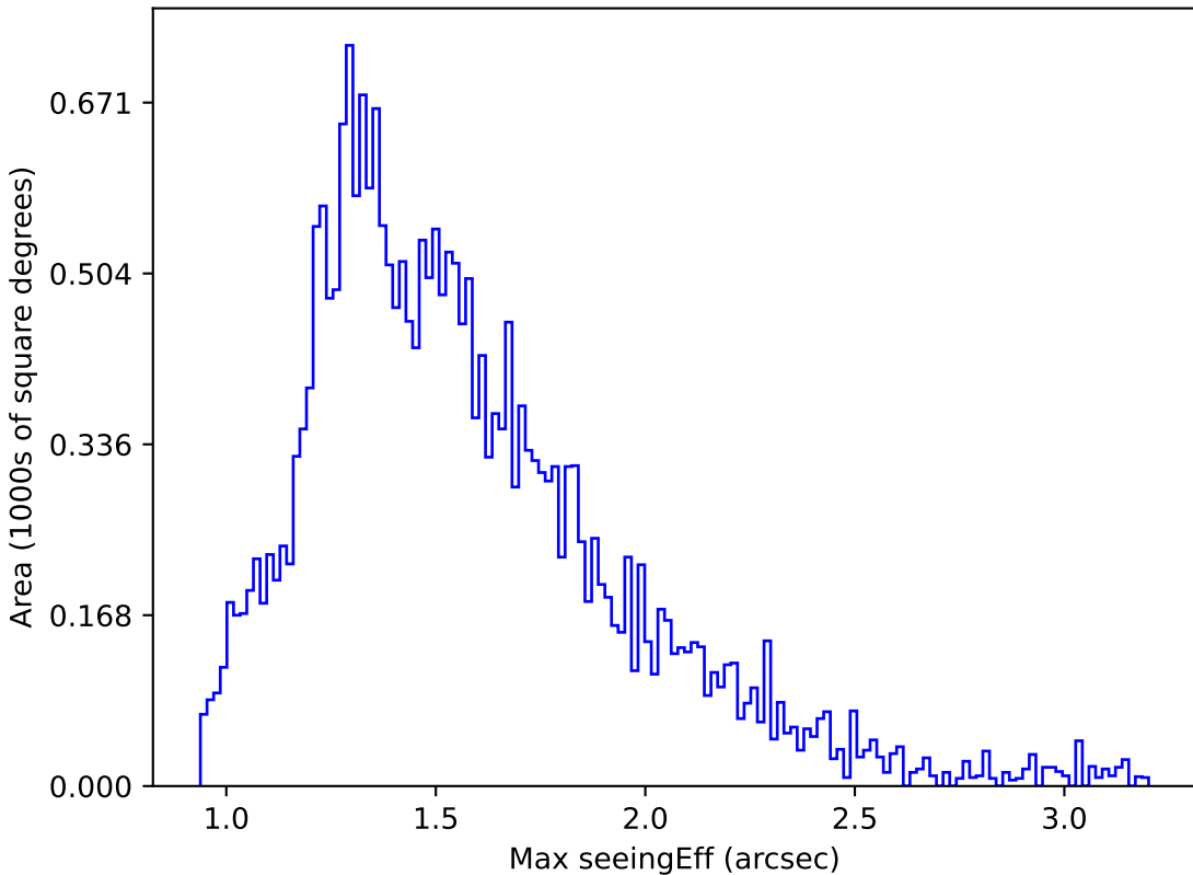
too_ignore_10_4v3.4_10yrs Yr 1 g band: Max seeingEff
