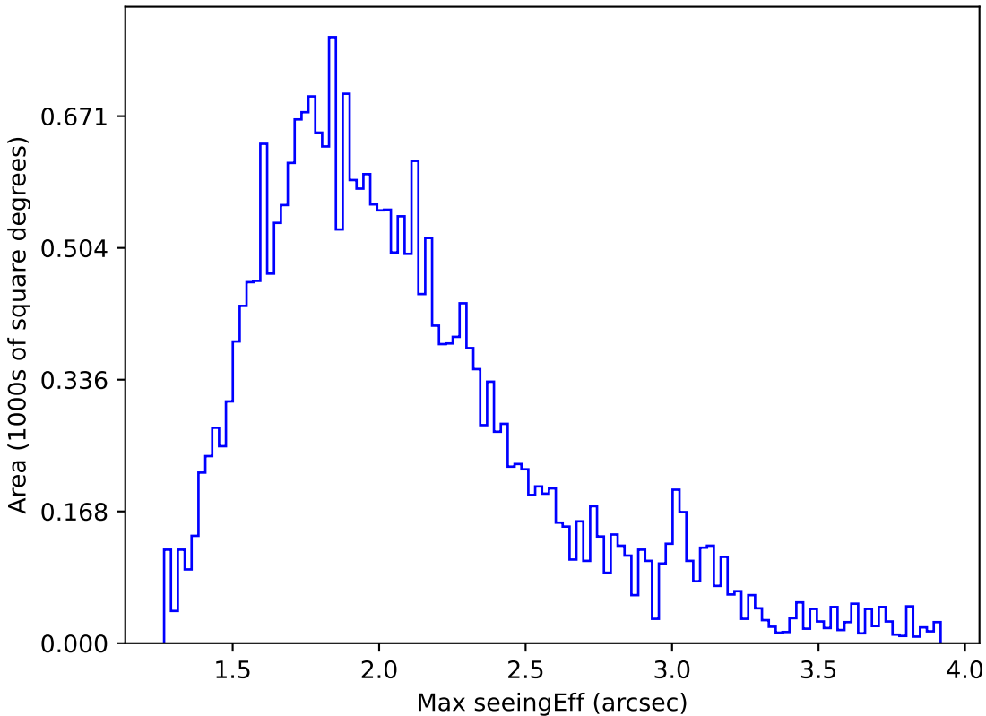
too_ignore_10_4v3.4_10yrs Yr 1 all bands: Max seeingEff
