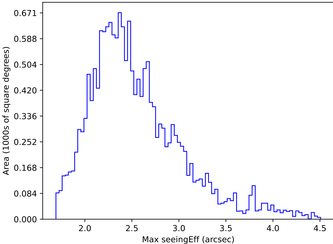
too_ignore_10_4v3.4_10yrs WFD z band: Max seeingEff
