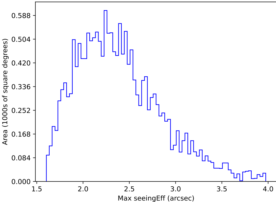
too_ignore_10_4v3.4_10yrs WFD y band: Max seeingEff
