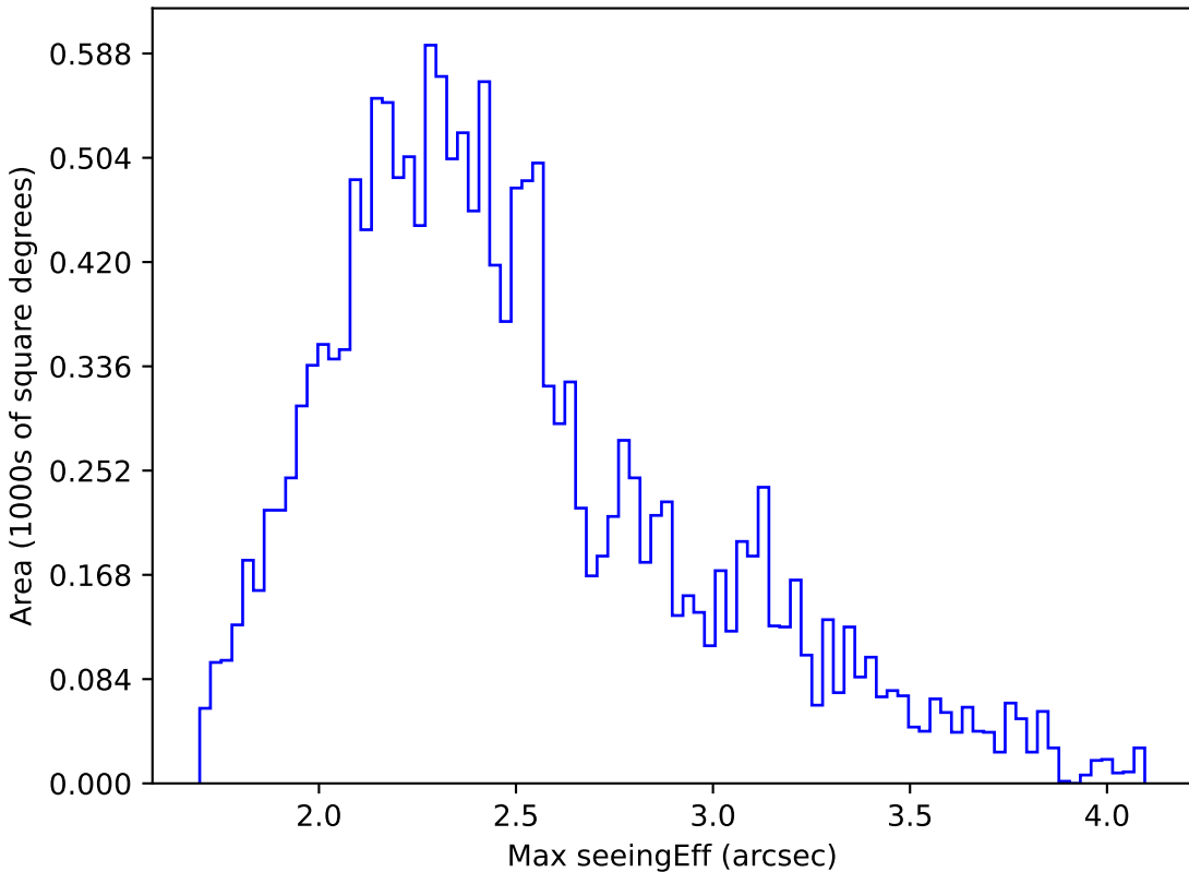
too_ignore_10_4v3.4_10yrs WFD u band: Max seeingEff
