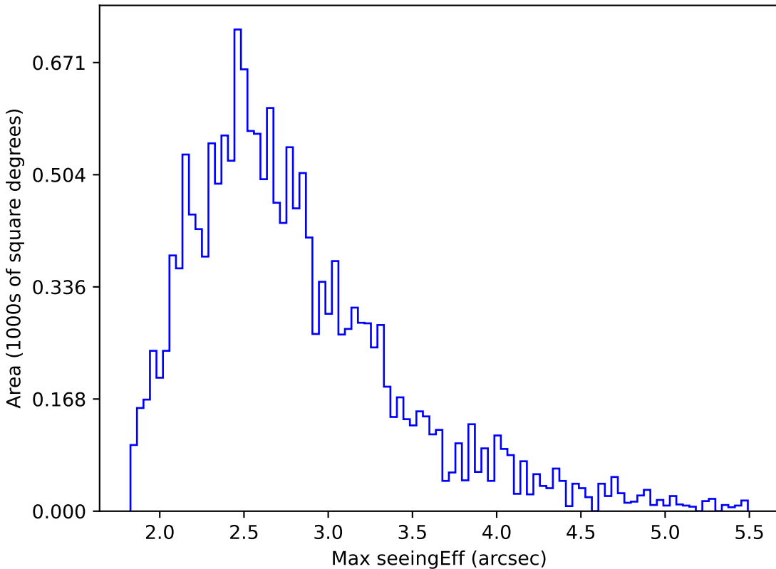
too_ignore_10_4v3.4_10yrs WFD r band: Max seeingEff
