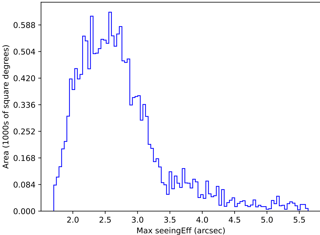
too_ignore_10_4v3.4_10yrs WFD i band: Max seeingEff
