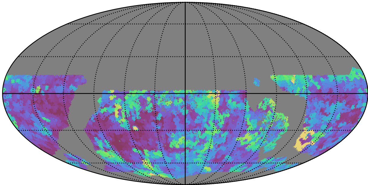
too_ignore_10_4v3.4_10yrs WFD g band: Max seeingEff
