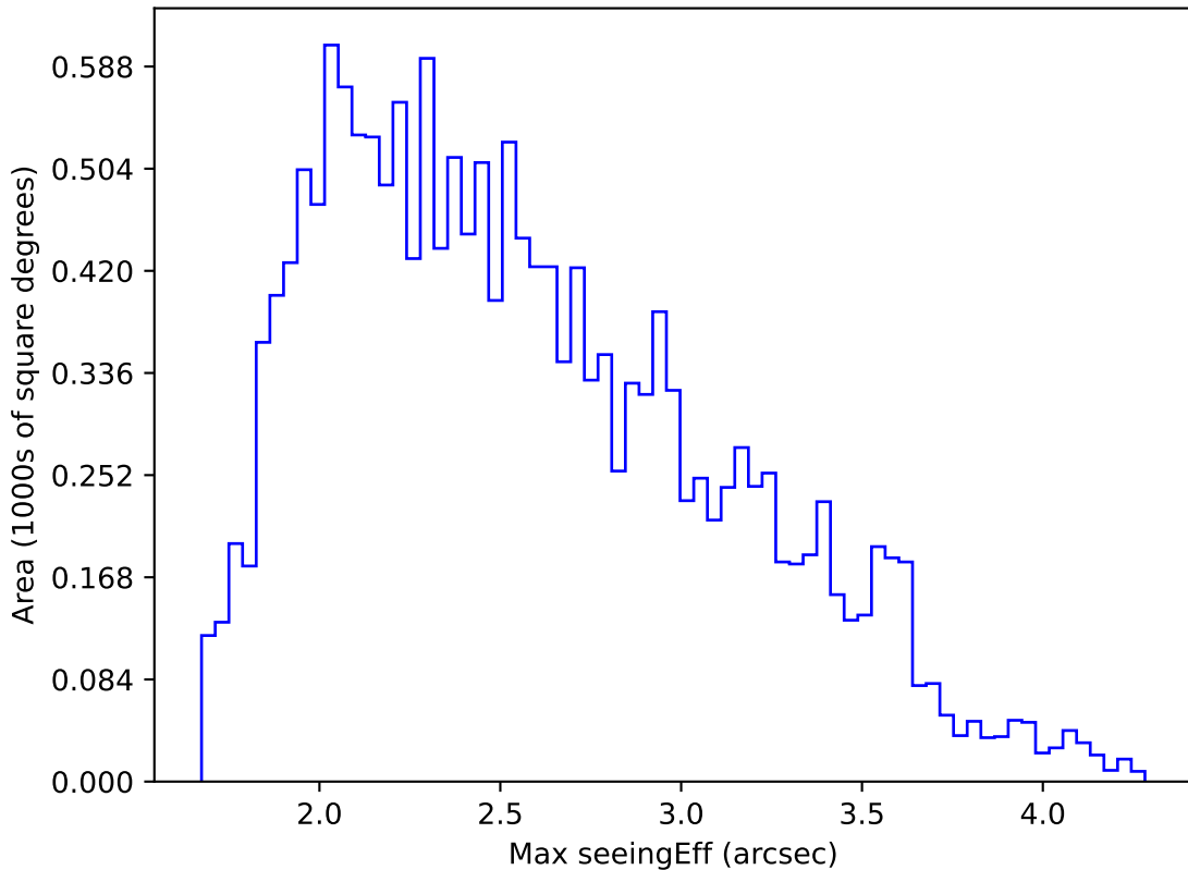
too_ignore_10_4v3.4_10yrs WFD g band: Max seeingEff
