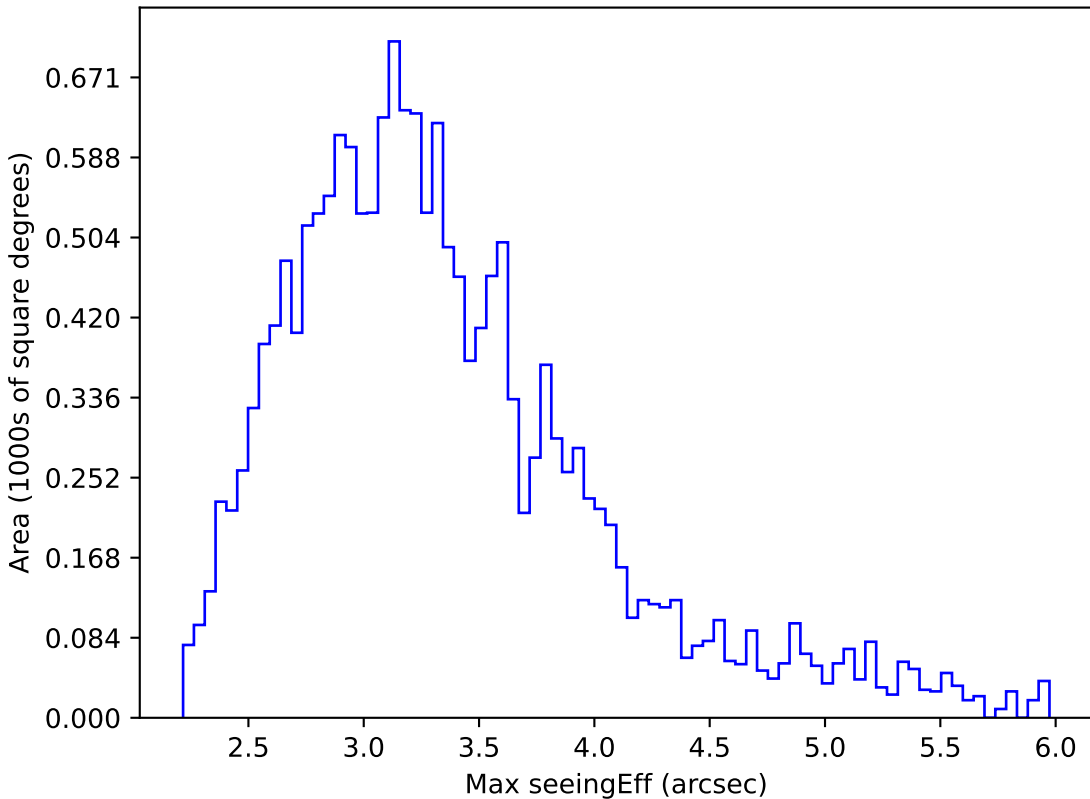
too_ignore_10_4v3.4_10yrs WFD all bands: Max seeingEff
