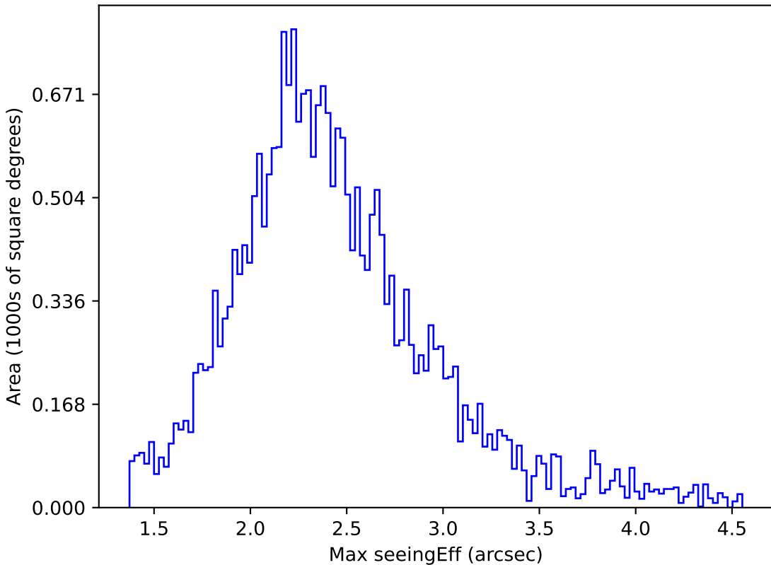
too_ignore_10_4v3.4_10yrs All sky z band: Max seeingEff
