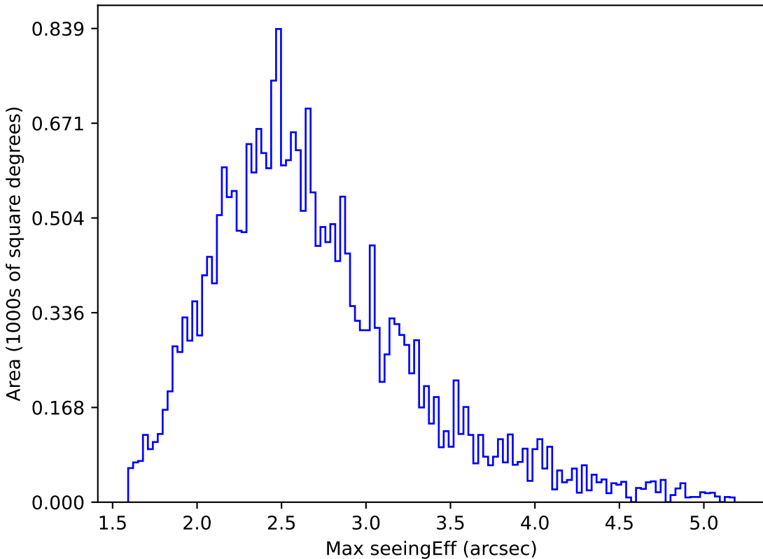
too_ignore_10_4v3.4_10yrs All sky r band: Max seeingEff
