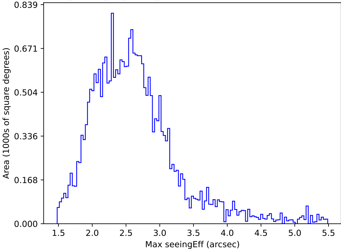
too_ignore_10_4v3.4_10yrs All sky i band: Max seeingEff
