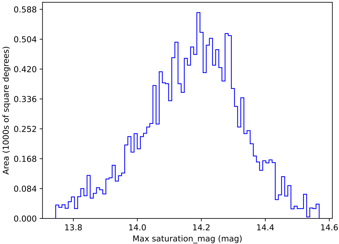
too_ignore_10_4v3.4_10yrs WFD y band: Max saturation_mag
