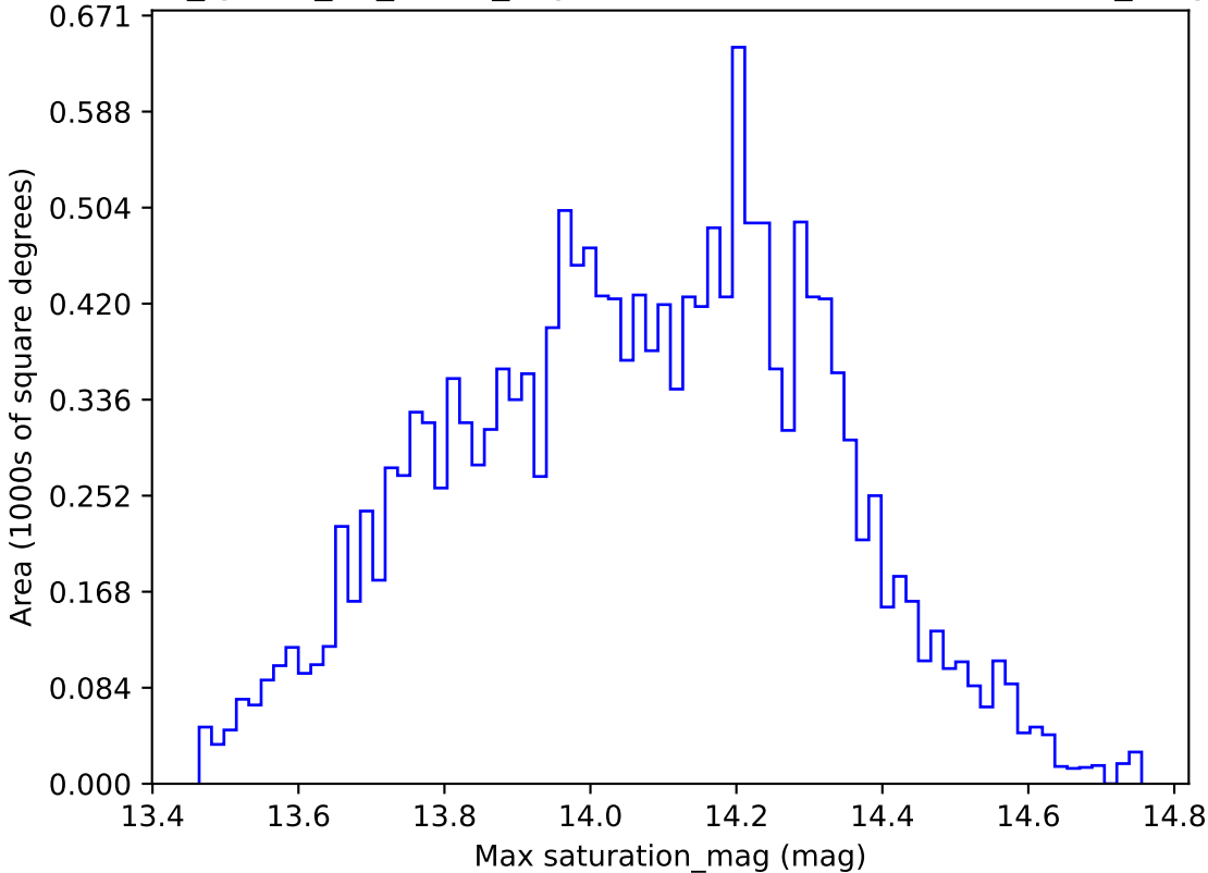
too_ignore_10_4v3.4_10yrs WFD u band: Max saturation_mag
