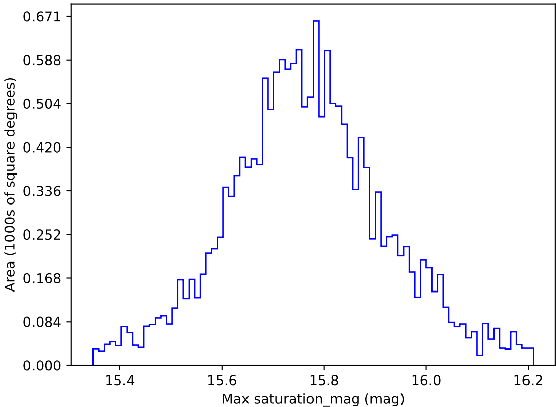
too_ignore_10_4v3.4_10yrs WFD r band: Max saturation_mag
