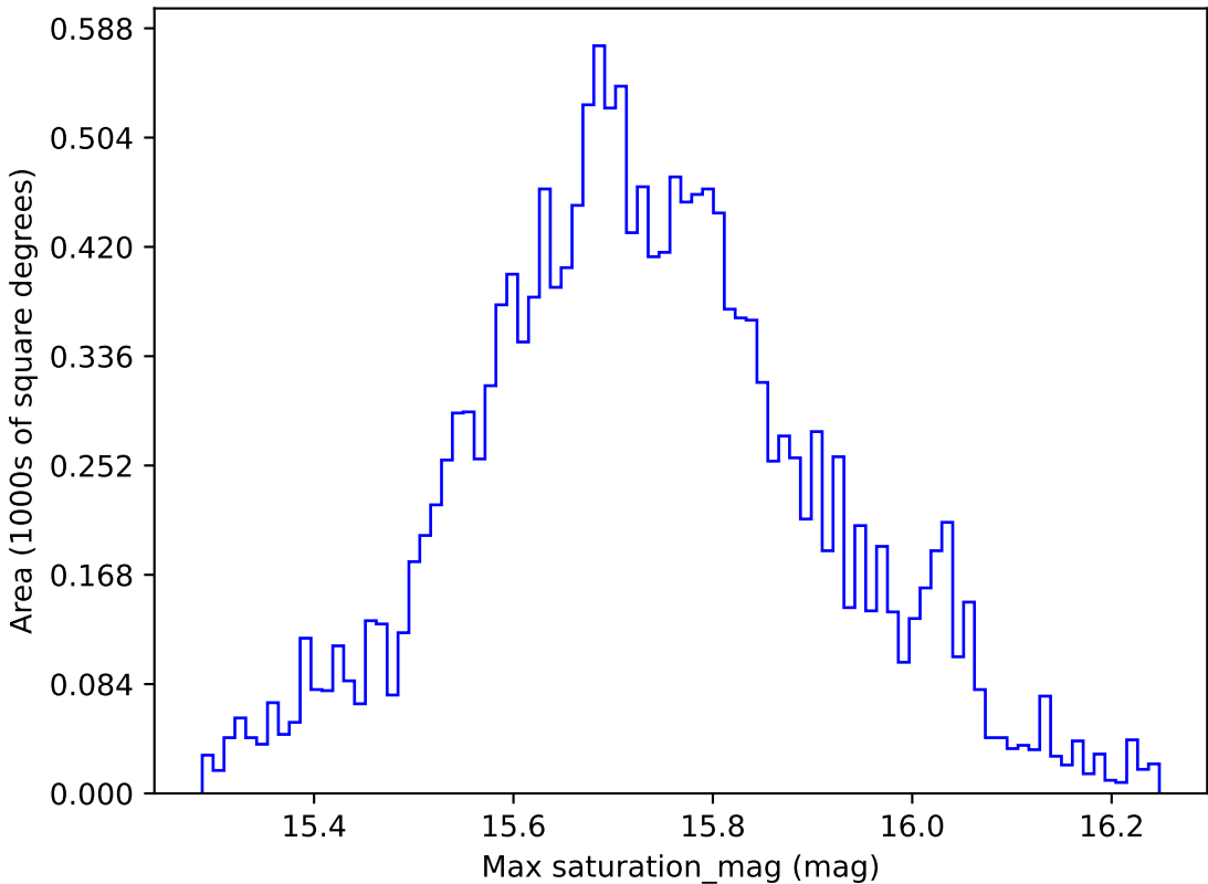
too_ignore_10_4v3.4_10yrs WFD g band: Max saturation_mag
