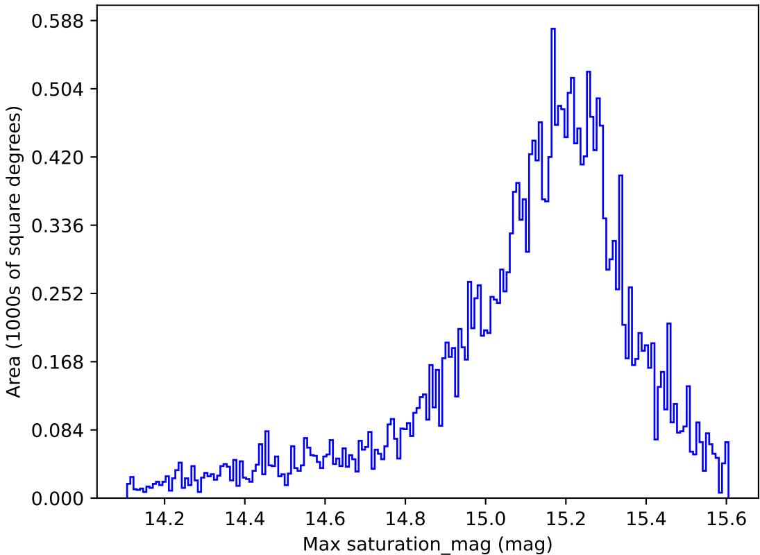
too_ignore_10_4v3.4_10yrs All sky z band: Max saturation_mag
