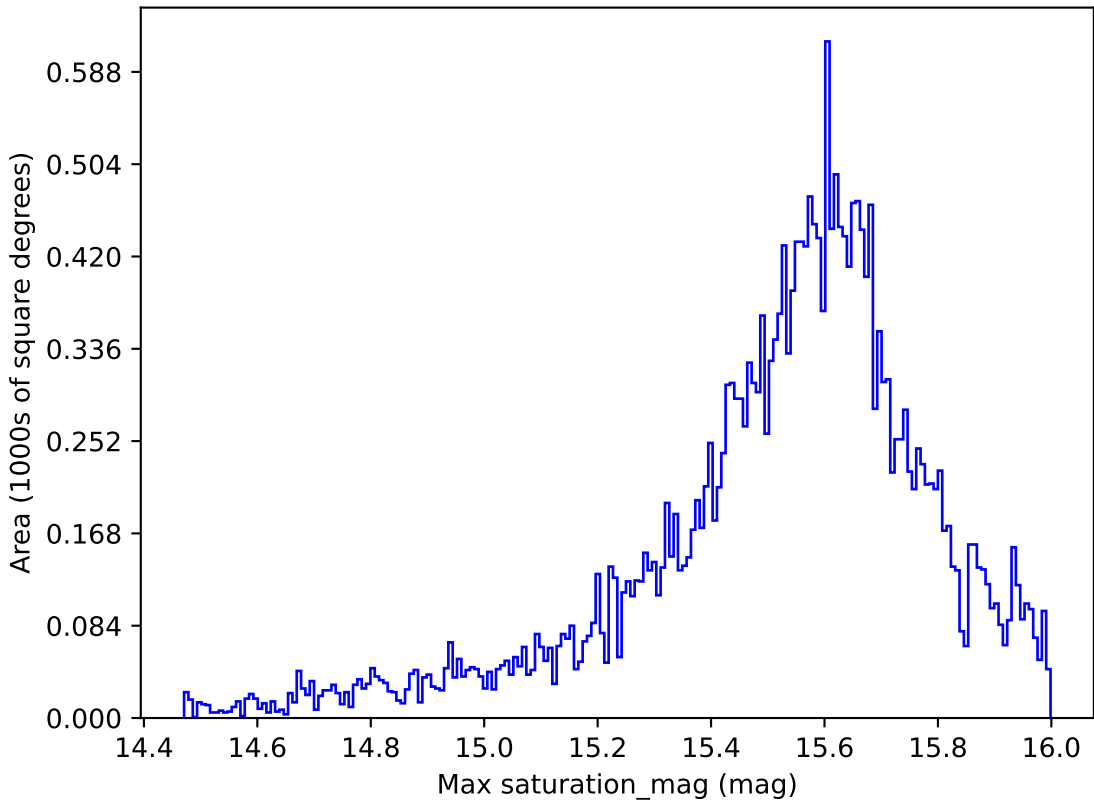
too_ignore_10_4v3.4_10yrs All sky i band: Max saturation_mag
