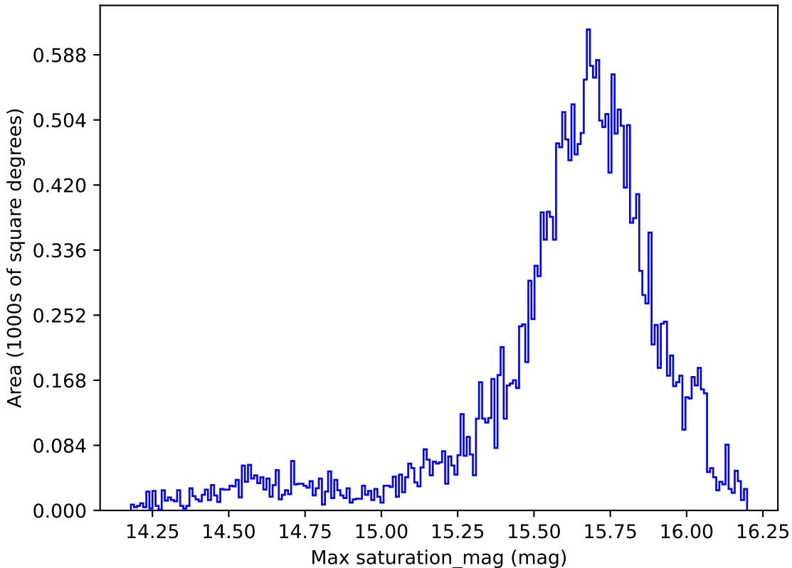
too_ignore_10_4v3.4_10yrs All sky g band: Max saturation_mag
