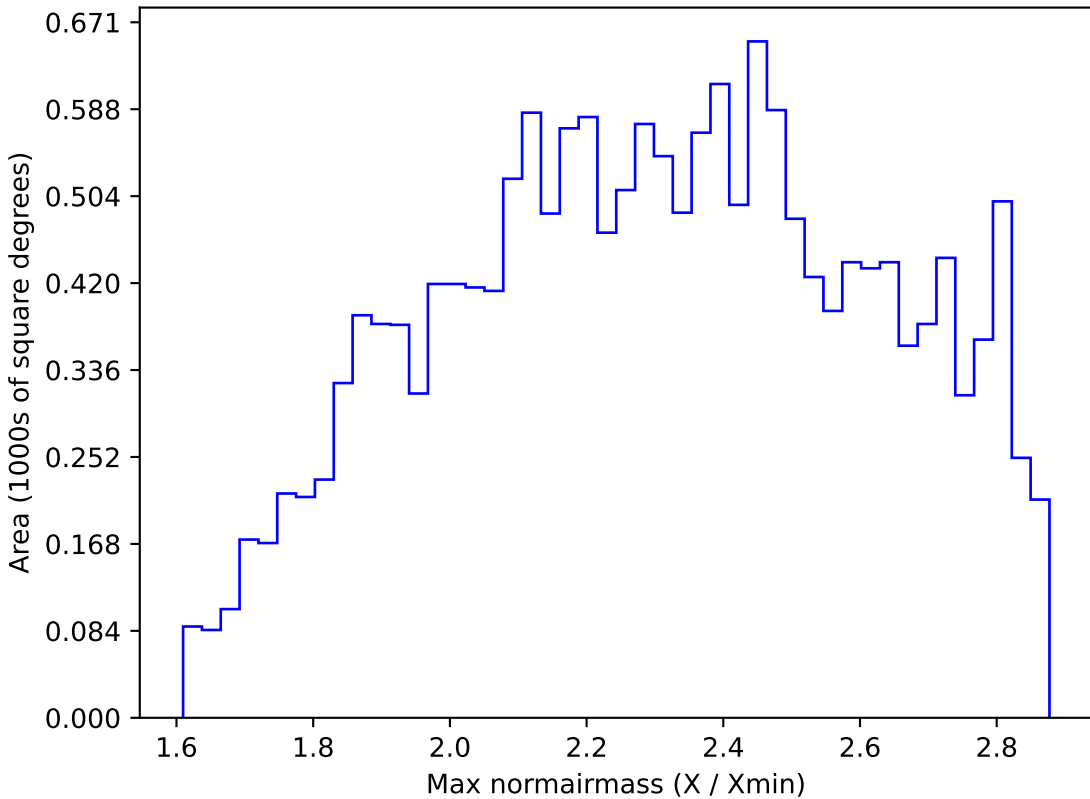
too_ignore_10_4v3.4_10yrs WFD z band: Max normairmass
