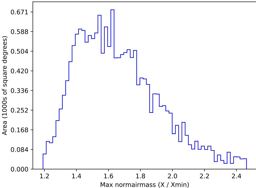
too_ignore_10_4v3.4_10yrs WFD u band: Max normairmass
