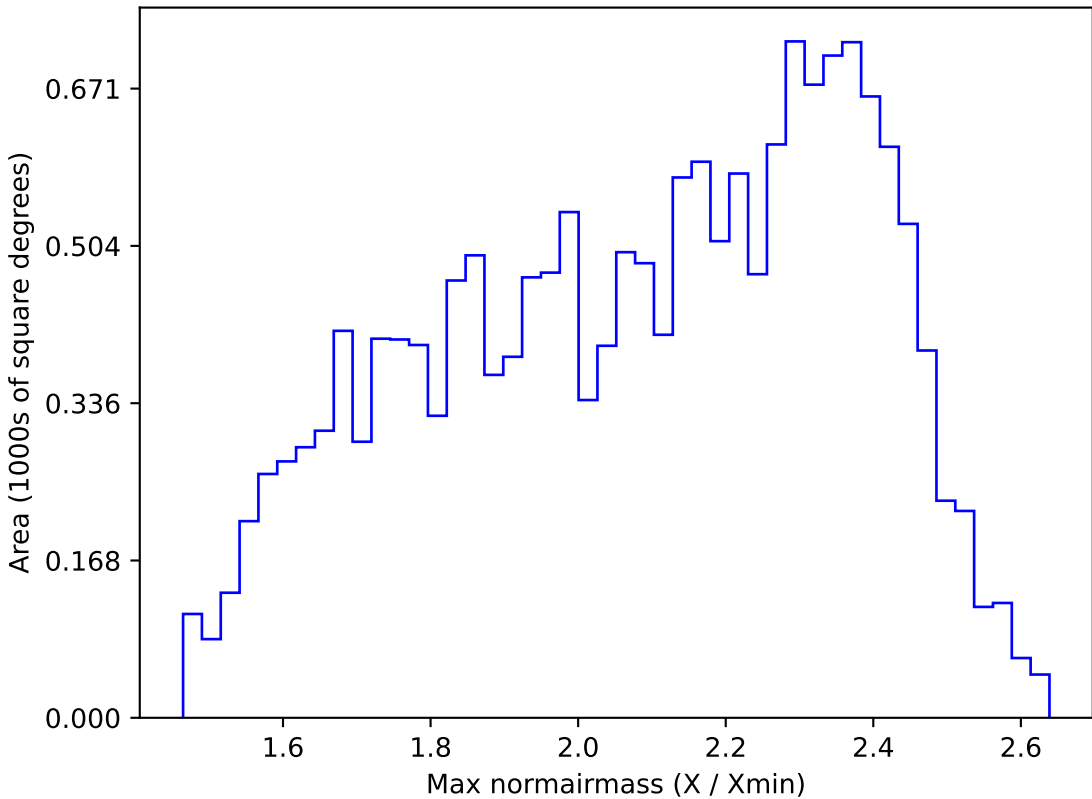
too_ignore_10_4v3.4_10yrs WFD r band: Max normairmass
