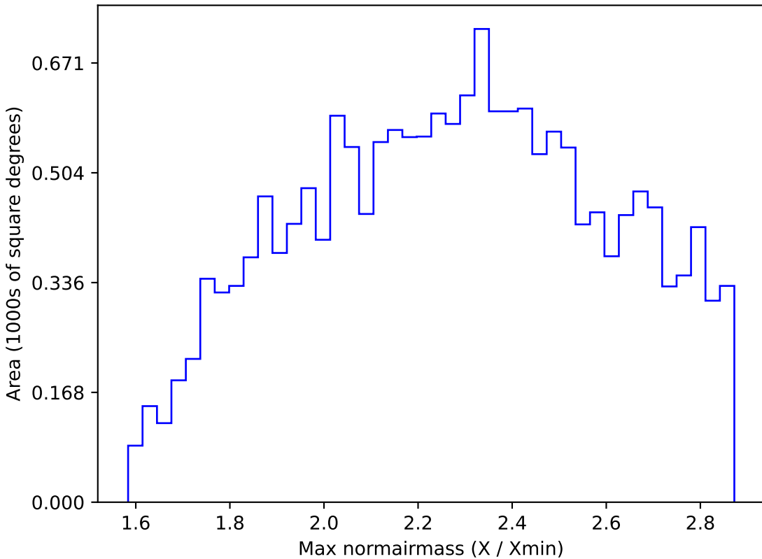
too_ignore_10_4v3.4_10yrs WFD i band: Max normairmass
