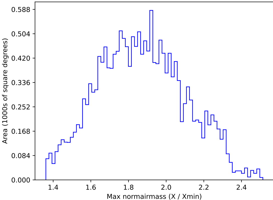
too_ignore_10_4v3.4_10yrs WFD g band: Max normairmass
