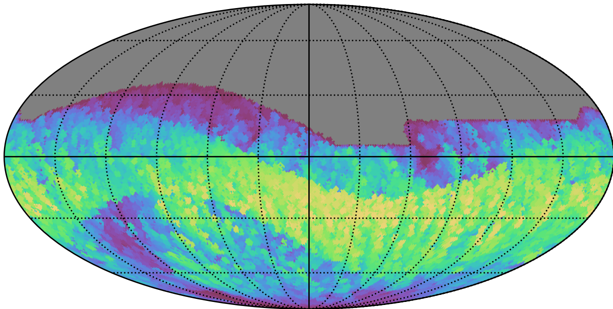
too_ignore_10_4v3.4_10yrs All sky z band: Max normairmass
