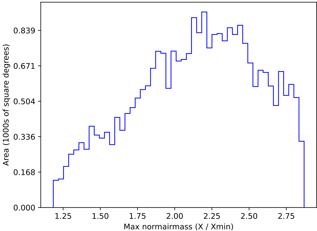
too_ignore_10_4v3.4_10yrs All sky z band: Max normairmass
