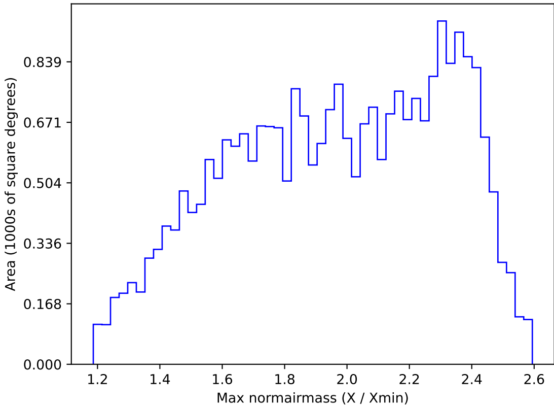
too_ignore_10_4v3.4_10yrs All sky r band: Max normairmass
