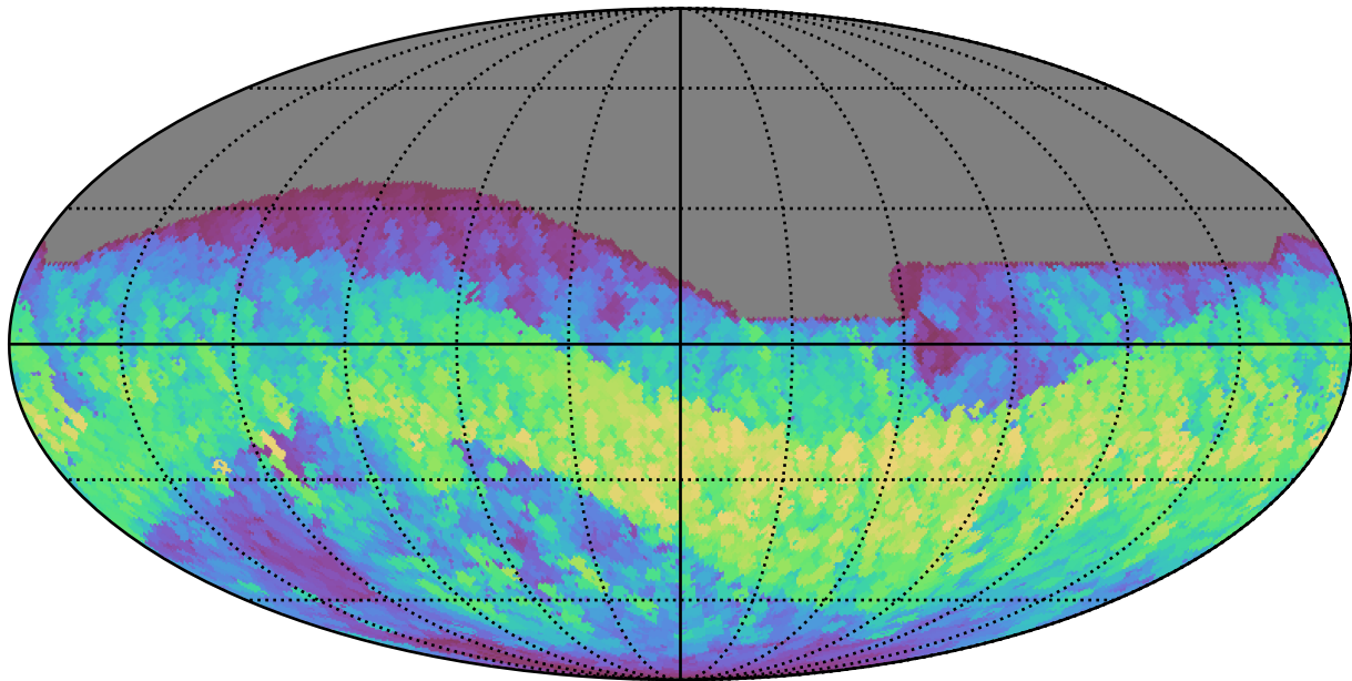
too_ignore_10_4v3.4_10yrs All sky i band: Max normairmass
