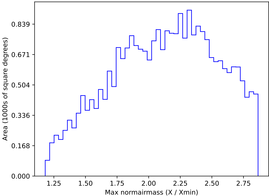
too_ignore_10_4v3.4_10yrs All sky i band: Max normairmass
