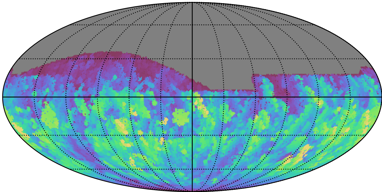
too_ignore_10_4v3.4_10yrs All sky g band: Max normairmass
