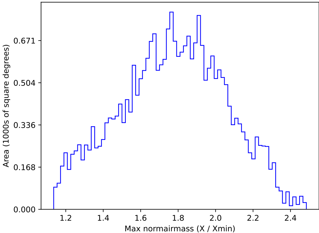
too_ignore_10_4v3.4_10yrs All sky g band: Max normairmass
