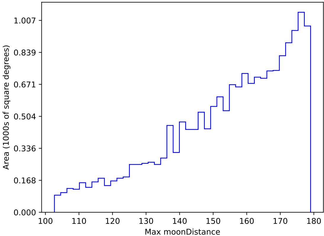
too_ignore_10_4v3.4_10yrs WFD z band: Max moonDistance
