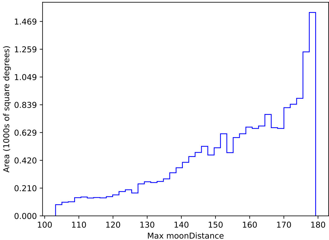
too_ignore_10_4v3.4_10yrs WFD r band: Max moonDistance
