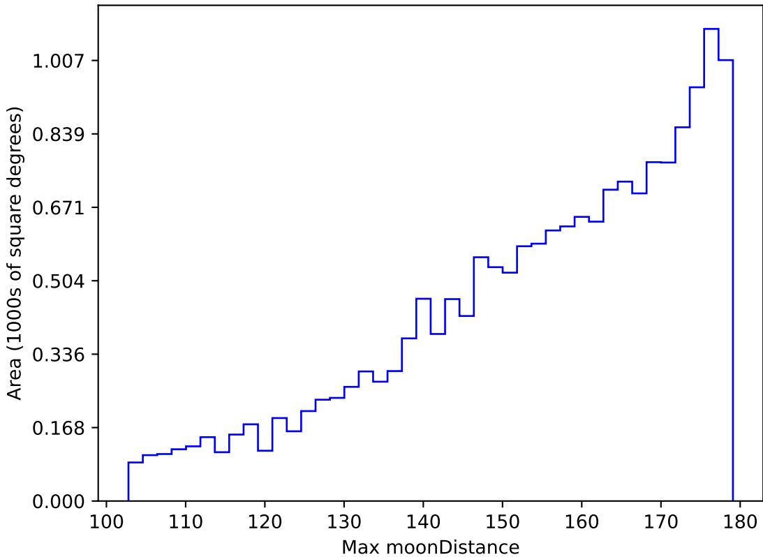
too_ignore_10_4v3.4_10yrs WFD g band: Max moonDistance
