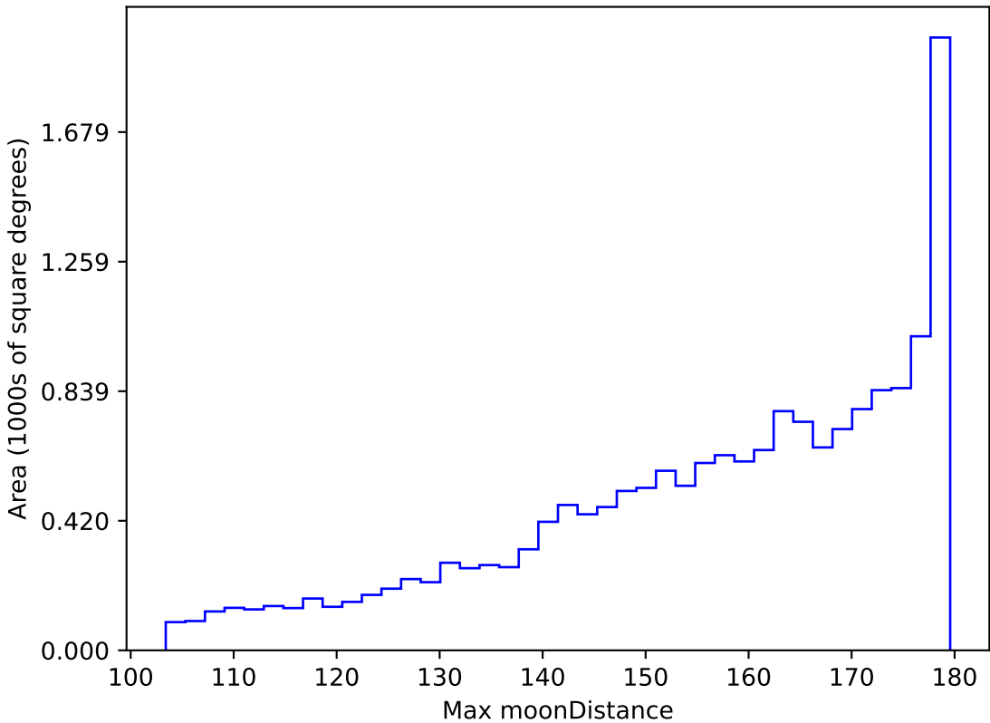
too_ignore_10_4v3.4_10yrs WFD all bands: Max moonDistance
