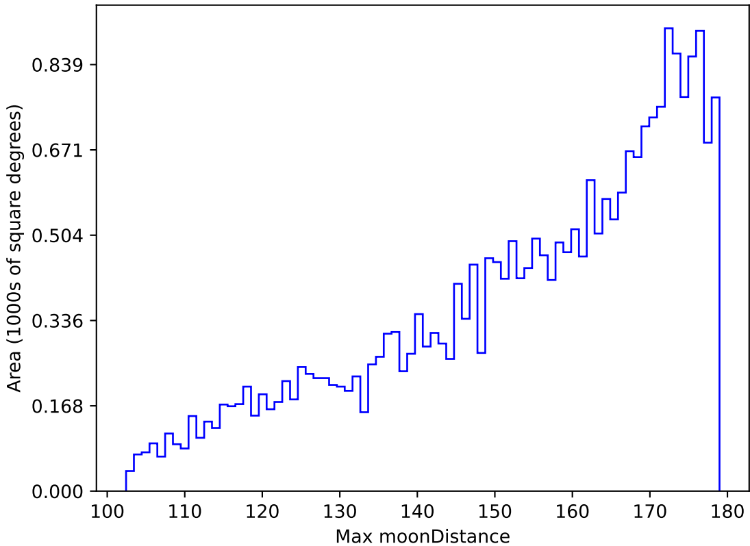
too_ignore_10_4v3.4_10yrs All sky z band: Max moonDistance
