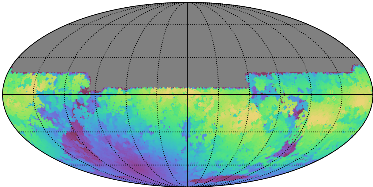
too_ignore_10_4v3.4_10yrs All sky y band: Max moonDistance
