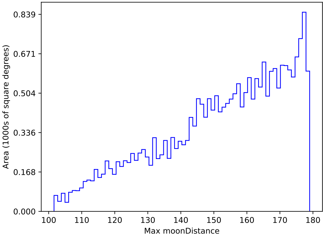
too_ignore_10_4v3.4_10yrs All sky u band: Max moonDistance
